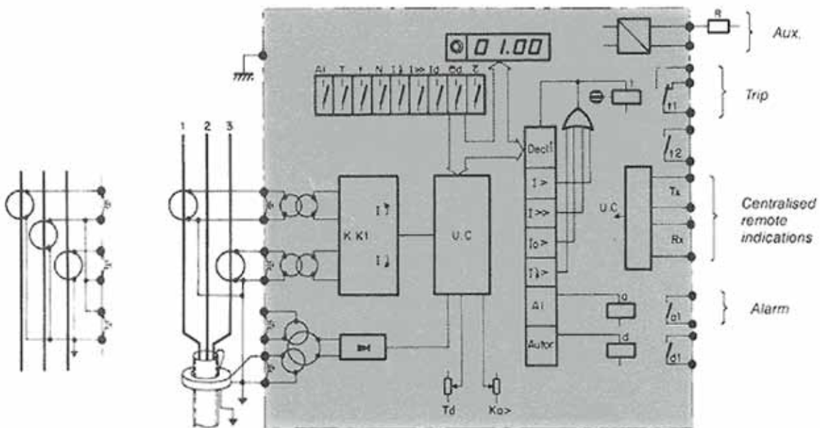
Fig. 3 - IMM 7990: Simplified operation and connection diagram
