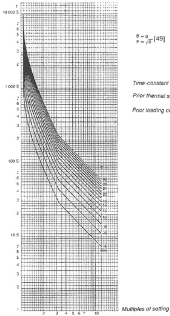
— Cold characteristics for different time constants.
