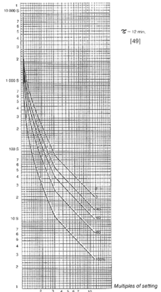
— 12 min time constant with different prior thermal states.
