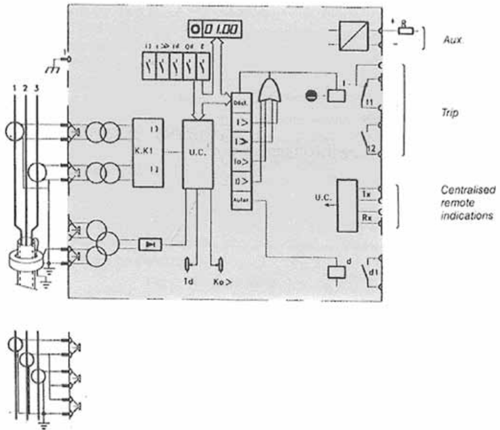
Fig. 2 - IMM 7960: Simplified operation and connection diagram
